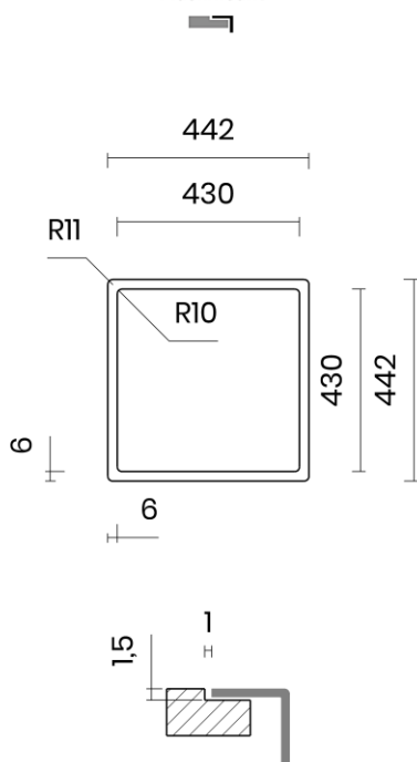
FILOTOP Flushmount
