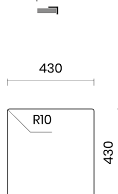
SOPRATOP Topmount
